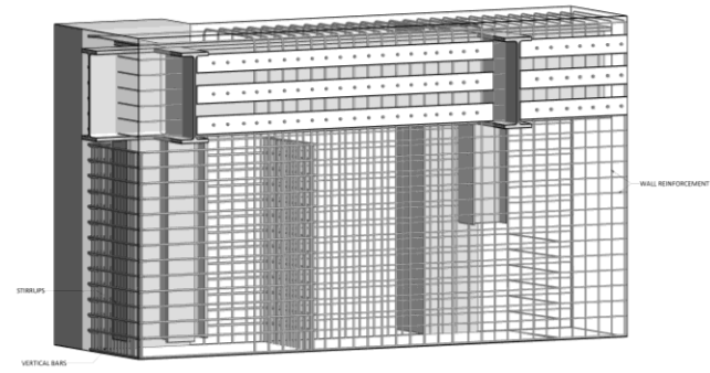
4 100 STEEL CONFINEMENT DETAIL (REINFORCEMENT)
