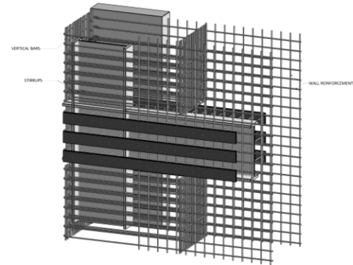
2 100 STEEL CONFINEMENT DETAIL (REINFORCEMENT)
