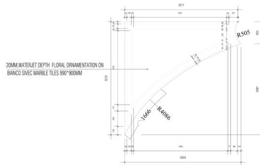
ID 01 DETAIL (01) 1:20
