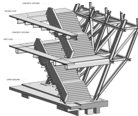
5 FEATURE STAIR WITH CONCRETE-3D VIEW 1:50
