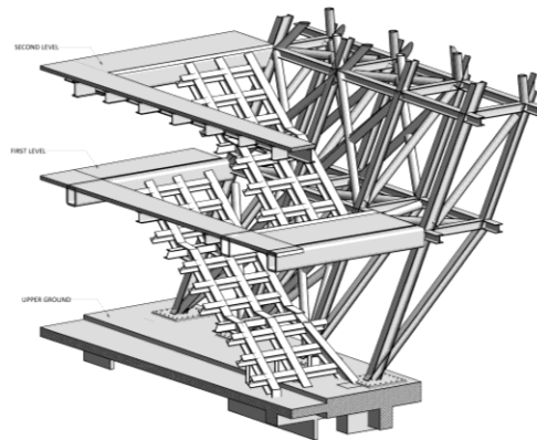
4 FEATURE STAIR-3D VIEW 1:50
