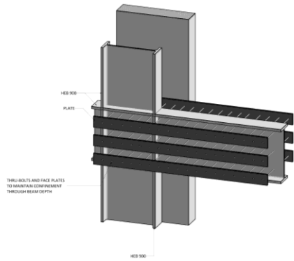
1 100 STEEL CONFINEMENT DETAIL (PLATE)
