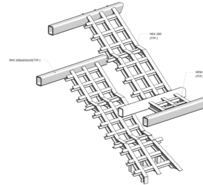
3 FEATURE STAIR STEEL SECTIONS 1:50
