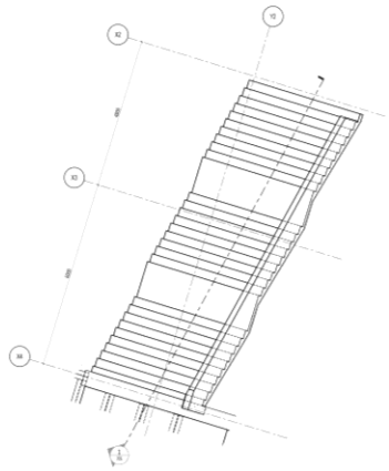
1 FEATURE STAIR PLAN AT UPPER GROUND 1:50
