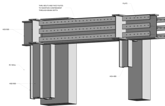
3 100 STEEL CONFINEMENT DETAIL (PLATE)
