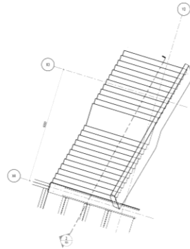
2 FEATURE STAIR PLAN AT FIRST FLOOR 1:50
